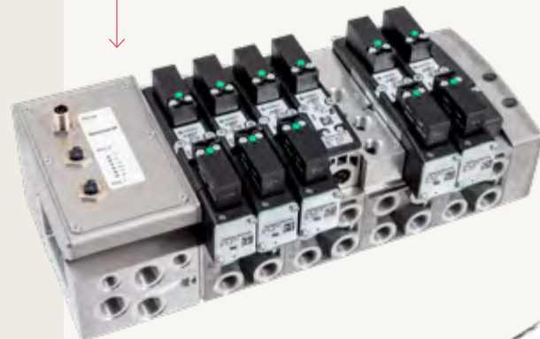
VS Series Valve Island
